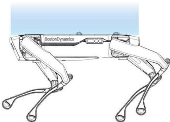
Vertical attachment zone (side view).
